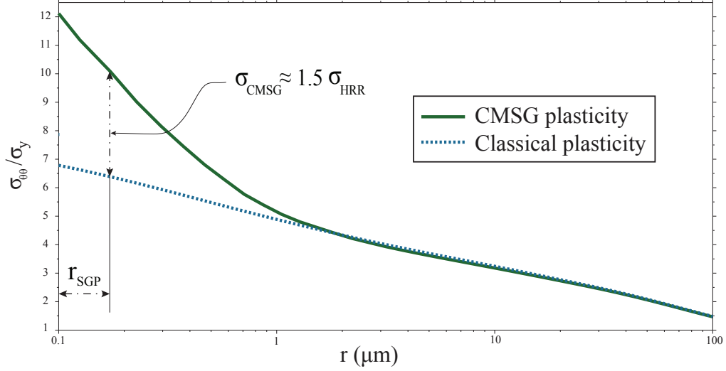
Figure 2: \sigma_{\theta\theta} distribution ahead of the crack tip for both MSG and classical plasticity theories in small strains, r being the distance to the crack tip in log scale for K_I = 17.3\sigma_Y\sqrt{l} , \sigma_Y = 0.2\% of E , \nu = 0.3 , N = 0.2 and l = 3.53 \mu\text{m}
