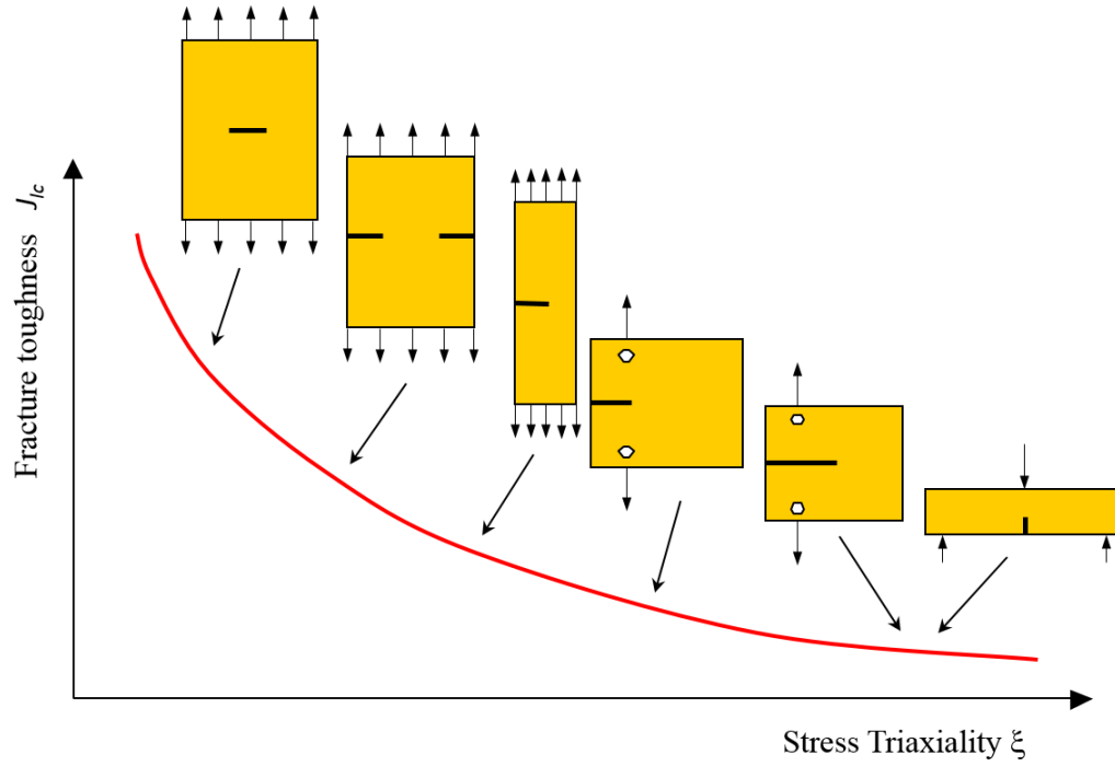
Figure 1: Influence of the specimen configuration on fracture toughness.
