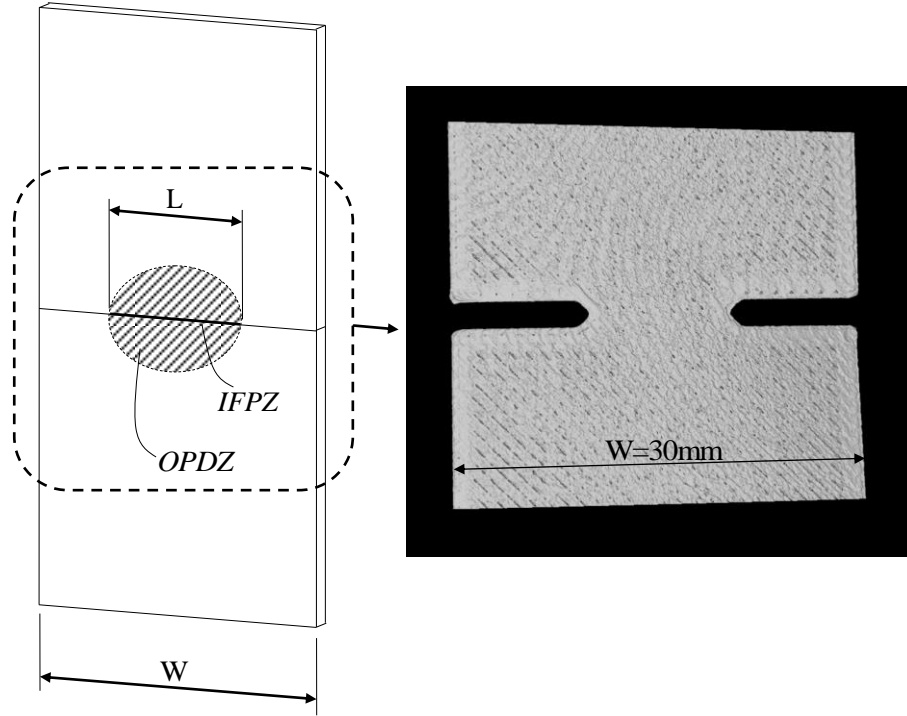
Figure 2. Deeply double edge notched tensile specimen. The outer process dissipation zone (OPDZ) and the inner fracture process zone (IFPZ) are marked.
