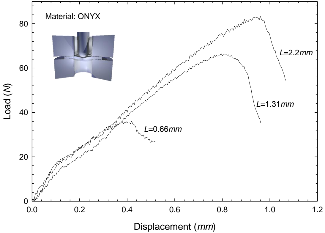
Figure 6. Load-displacement curves obtained from DDEN-SP specimens for Onyx.
