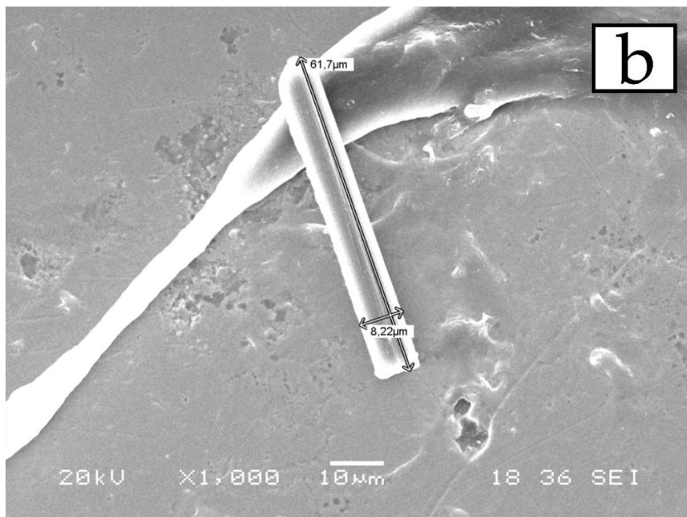
Figure 1. Aspect of the short fibres embedded in the nylon matrix: (a) general view, and (b) detailed view.
