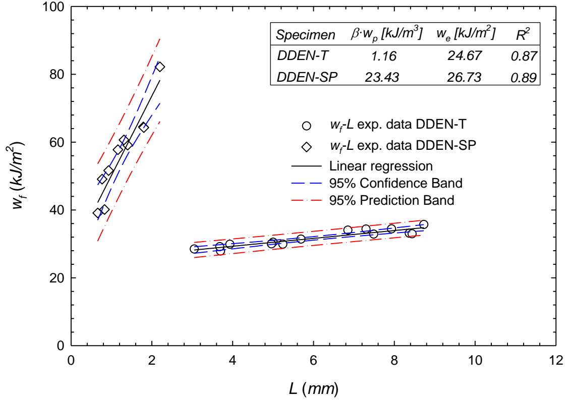
Figure 8. Specific work of fracture, w_f , versus ligament length L . Comparison of the EWF results obtained for DDEN-T and DDEN-SP experiments on a fibre-reinforced polymer (Onyx).
