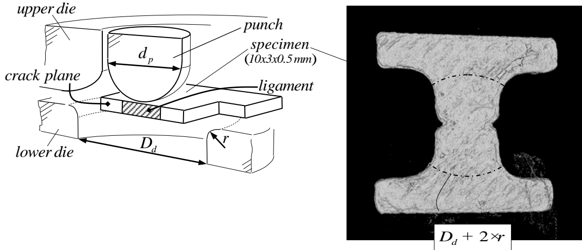
Figure 3. Small punch test device and DDEN-SP specimen.
