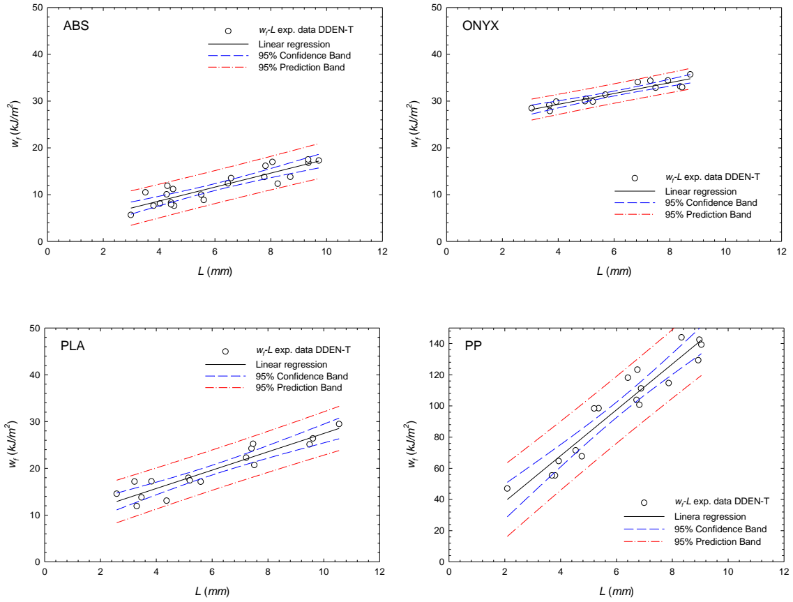
Figure 5. Specific work of fracture obtained from the DDEN-T specimens for, respectively, ABS, Onyx, PLA and PP. The linear regression of the data, along with the 95% confidence and prediction bands are also shown.
