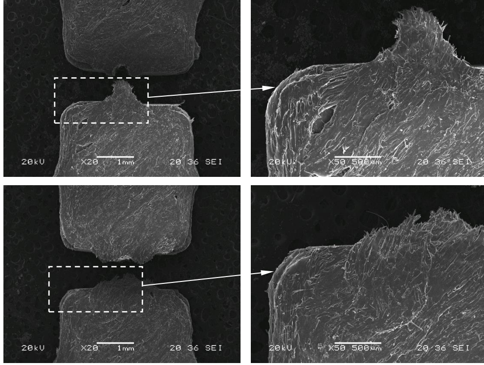
Figure 7. Detail images of the fracture process in deeply double edge notched small punch specimens for Onyx.
