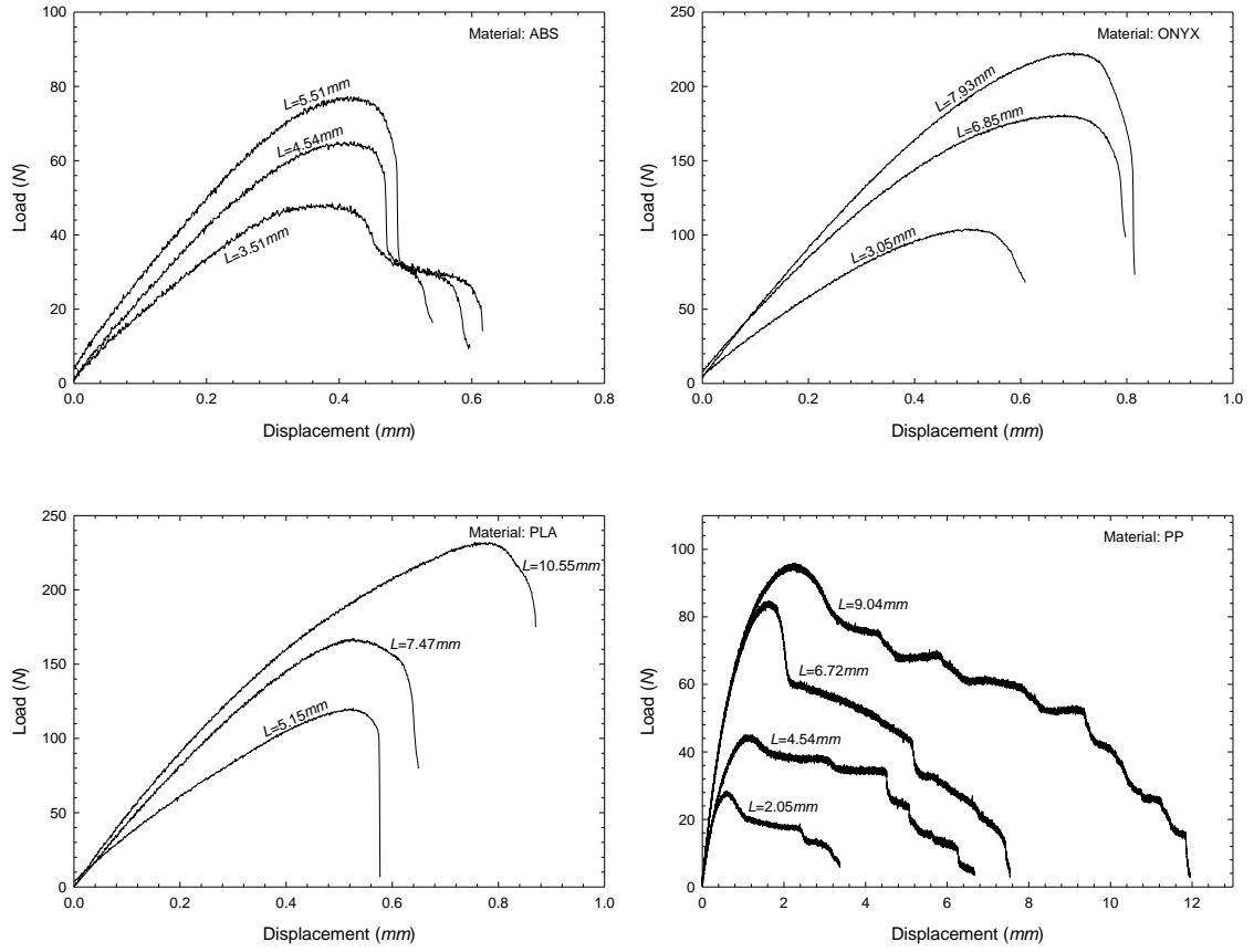
Figure 4. Load-displacement curves obtained from the DDEN-T specimens for, respectively, ABS, Onyx, PLA and PP.
